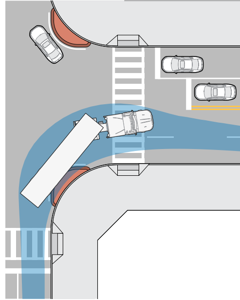
Figure 10. Mountable truck apron
