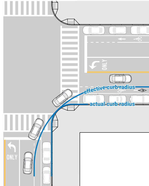
Figure 12. Actual vs. effective curb radius
