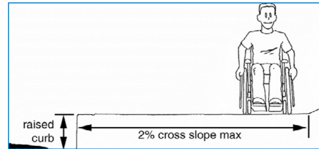
Figure 18. This sidewalk does not exceed 2 percent cross slope, ensuring that people using mobility devices will not tip over on their left or right side. Credit: US Access Board
