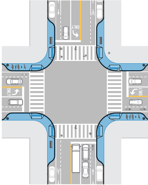
Figure 9. Curb extensions
