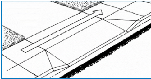
Figure 19. A sidewalk at the back of a driveway creates a level pedestrian route, meeting the proposed ADA cross slope requirement of 2 percent or less. Credit: US Access Board
