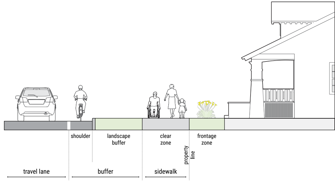
Figure 3. Functional Zones in a Medium- to Low-Density Residential Environment
