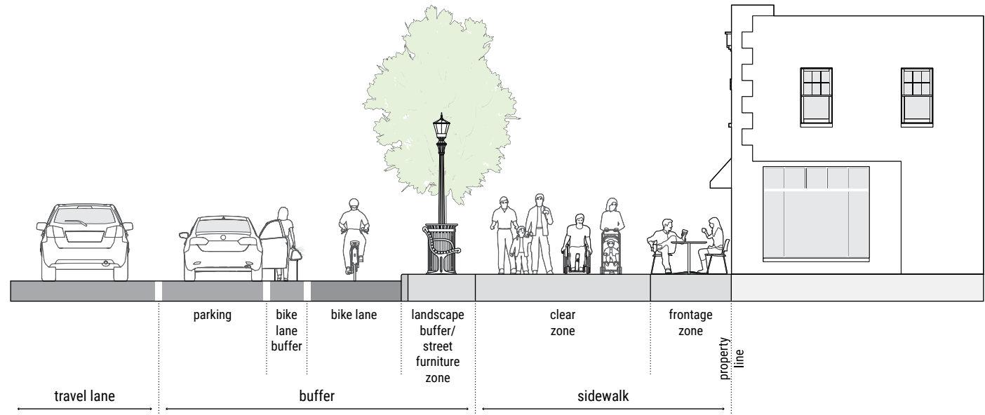
Figure 4. Functional Zones in a Town or Village Center Mixed-Use Environment
